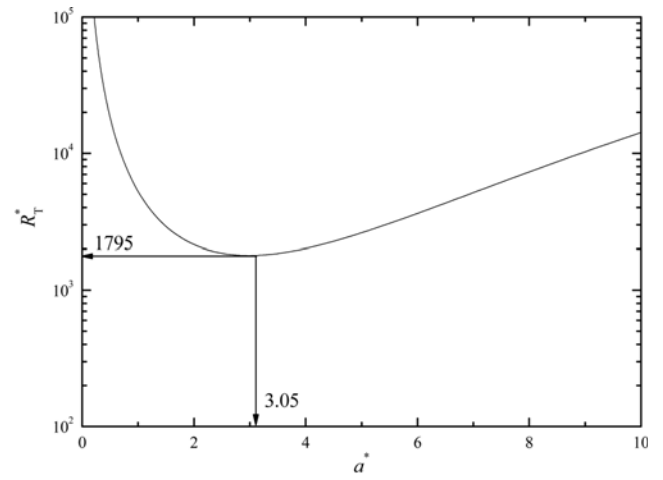
Fig. 2. Marginal stability curve for \text{Pr}=1 , \lambda=1 , \alpha_r=1 and k_r=1 .
